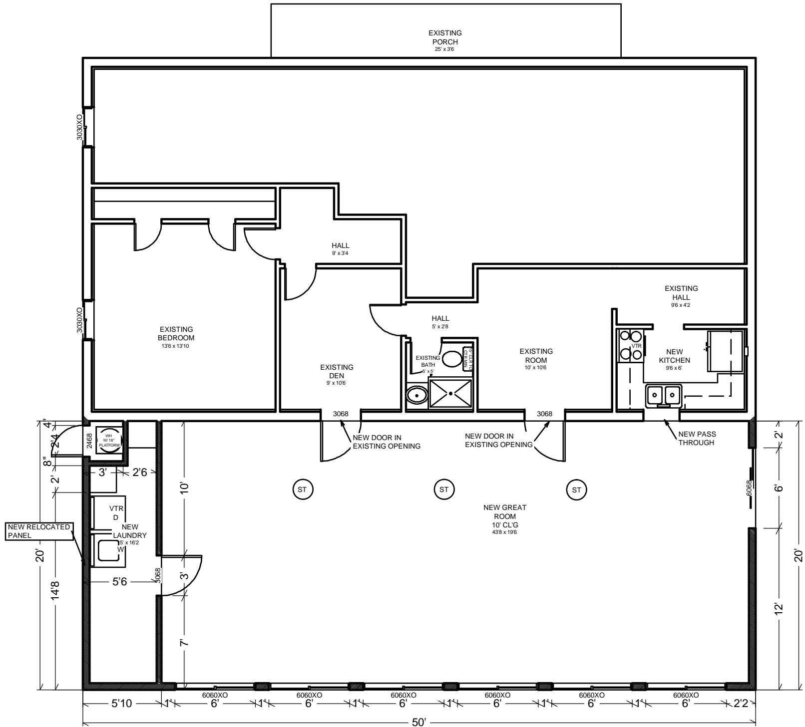
NEW FLOOR PLAN
